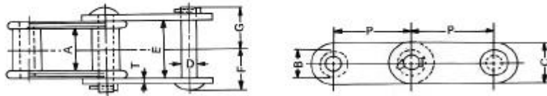
"C" Class Combination Chains
