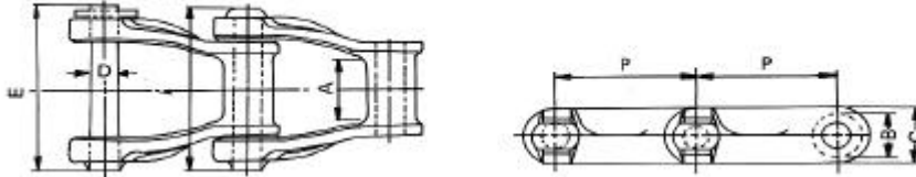
"H" Class Mill Chains
