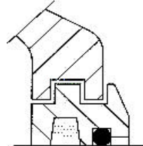
TS-UF seal, TS5xxUF
