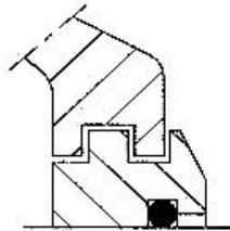
TS-U seal, TS5xxU
