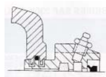
TER seal for SAF/SDAF
