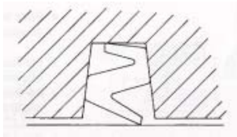
ZF seal for SN/SD
