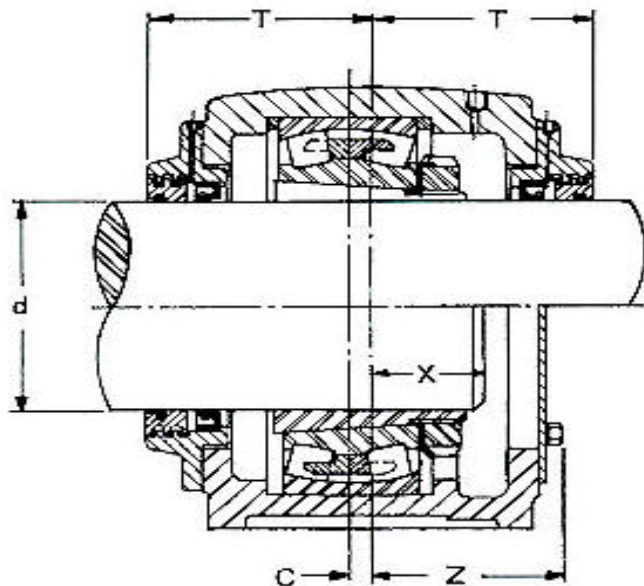
TACONITE TYPE SEAL (TAC SEAL)
