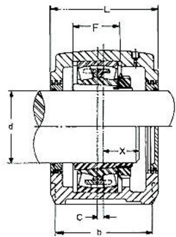
TRIPLE "TS" SEAL STANDARD ON SD HOUSINGS
